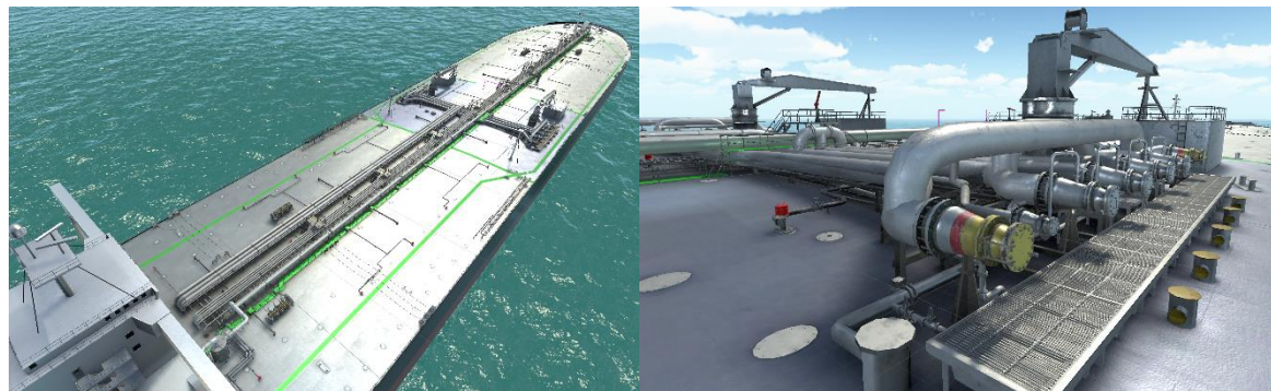
3D visualization of the cargo deck with areas indicating that local operational training is possible
